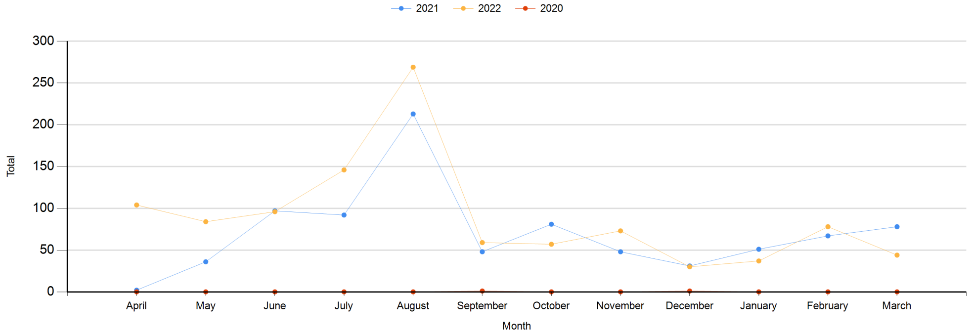
Trendline Between 01/04/2020 - 31/03/2023
